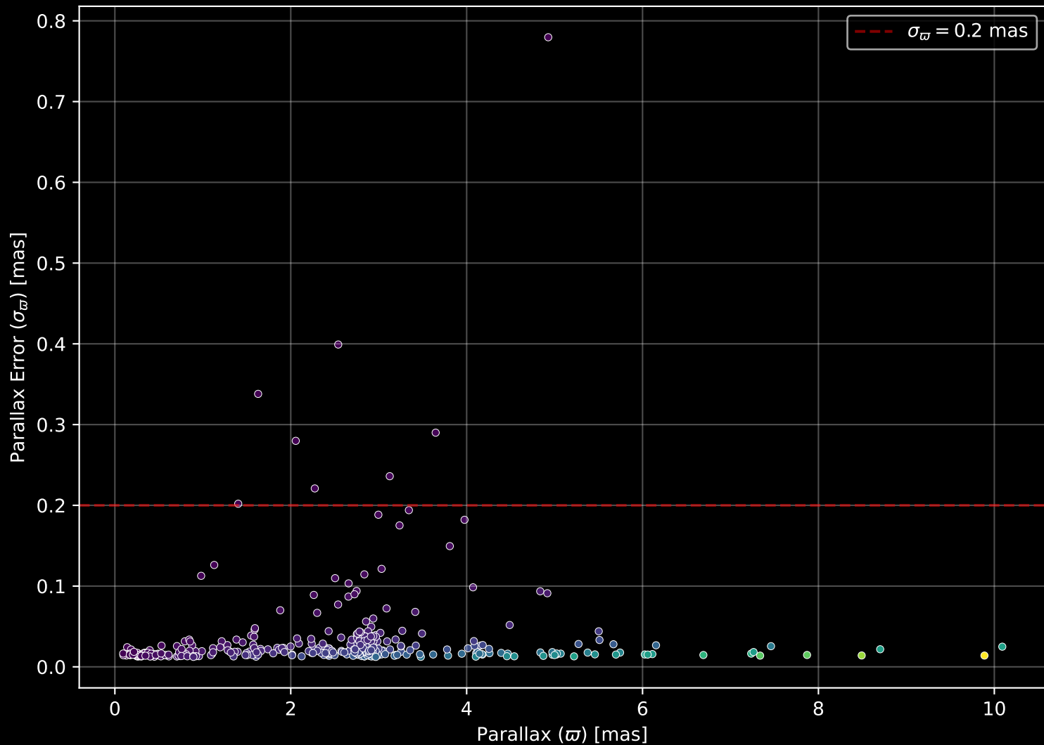
APOGEE DR17 Field: [ORIONOB1AB-E] Parallax Quality (n= 412)
