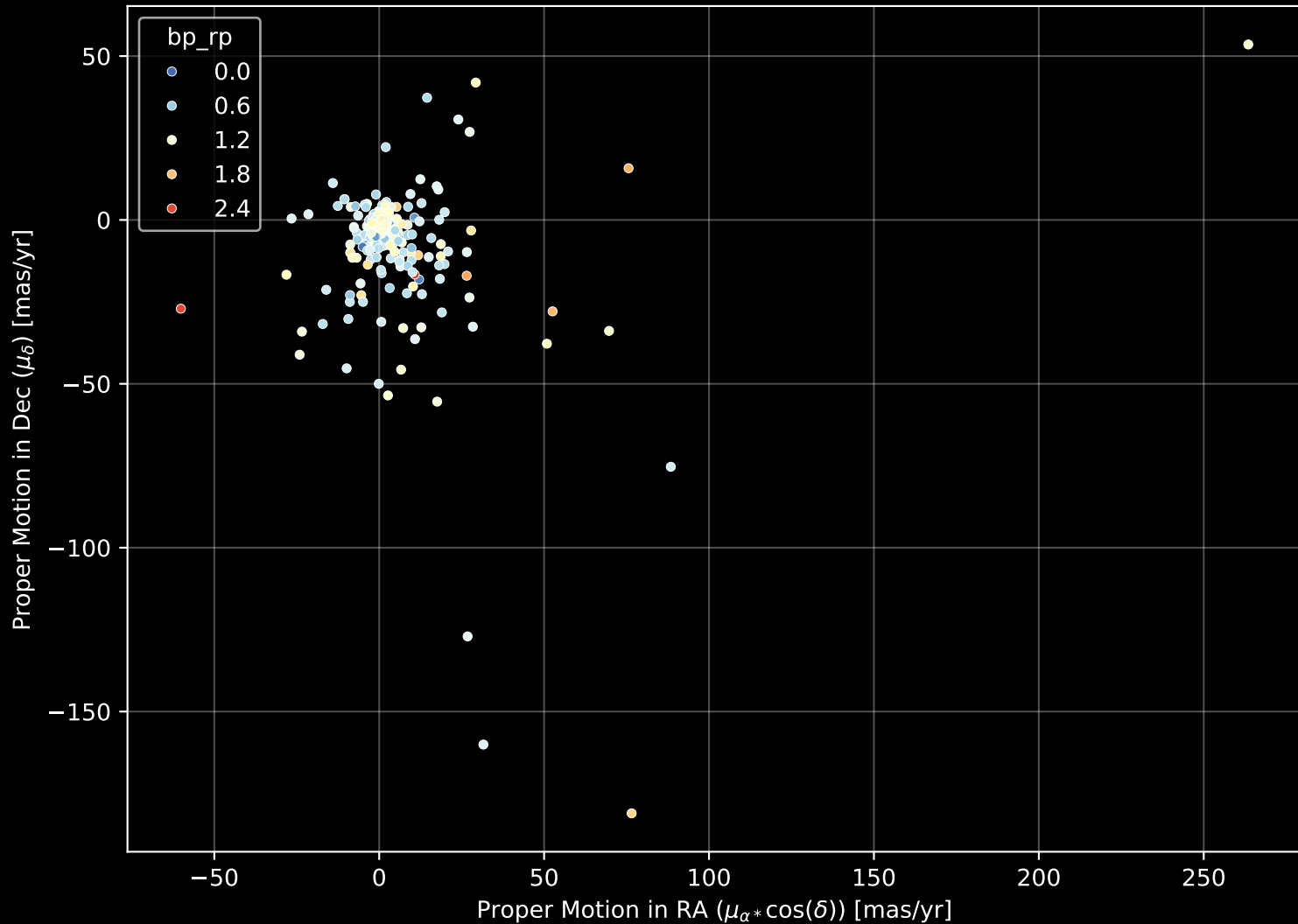
APOGEE DR17 Field: [ORIONOB1AB-E] Proper Motion Diagram (n= 412)
