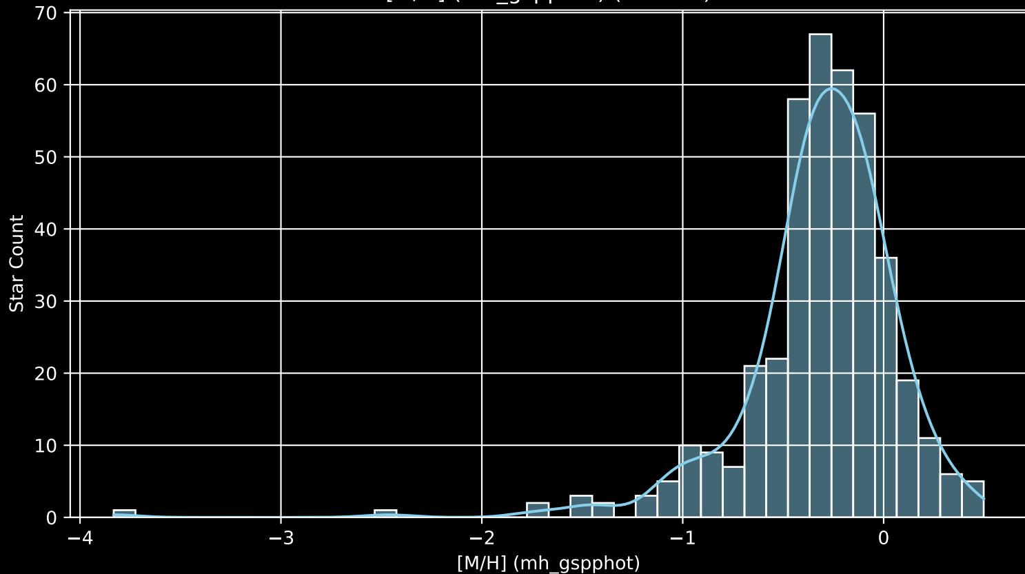
APOGEE DR17 Field: [ORIONOB1AB-E [M/H] (mh_gspphot) (n= 406)
