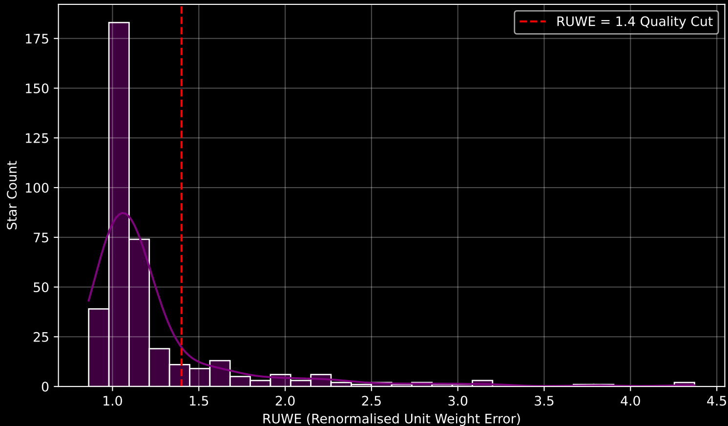
GAPOGEE DR17 Field [ORIONOB1AB-E] RUWE Distribution (n= 388)
