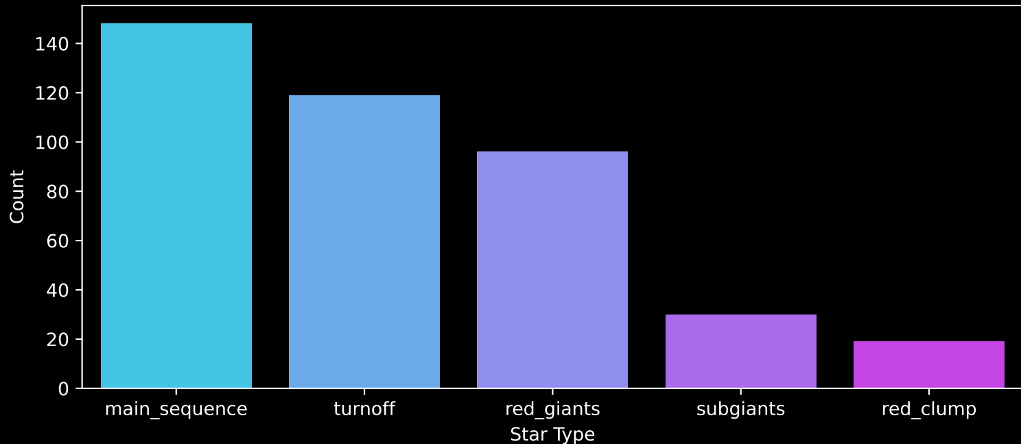
APOGEE DR17 Field: [ORIONOB1AB-E] Count plot of Star Type
