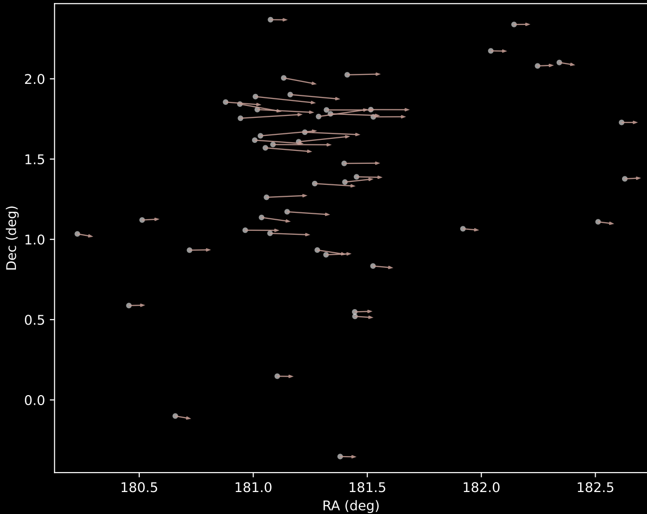
APOGEE DR17 Cluster 11 Proper Motion Vectors (n=49)
