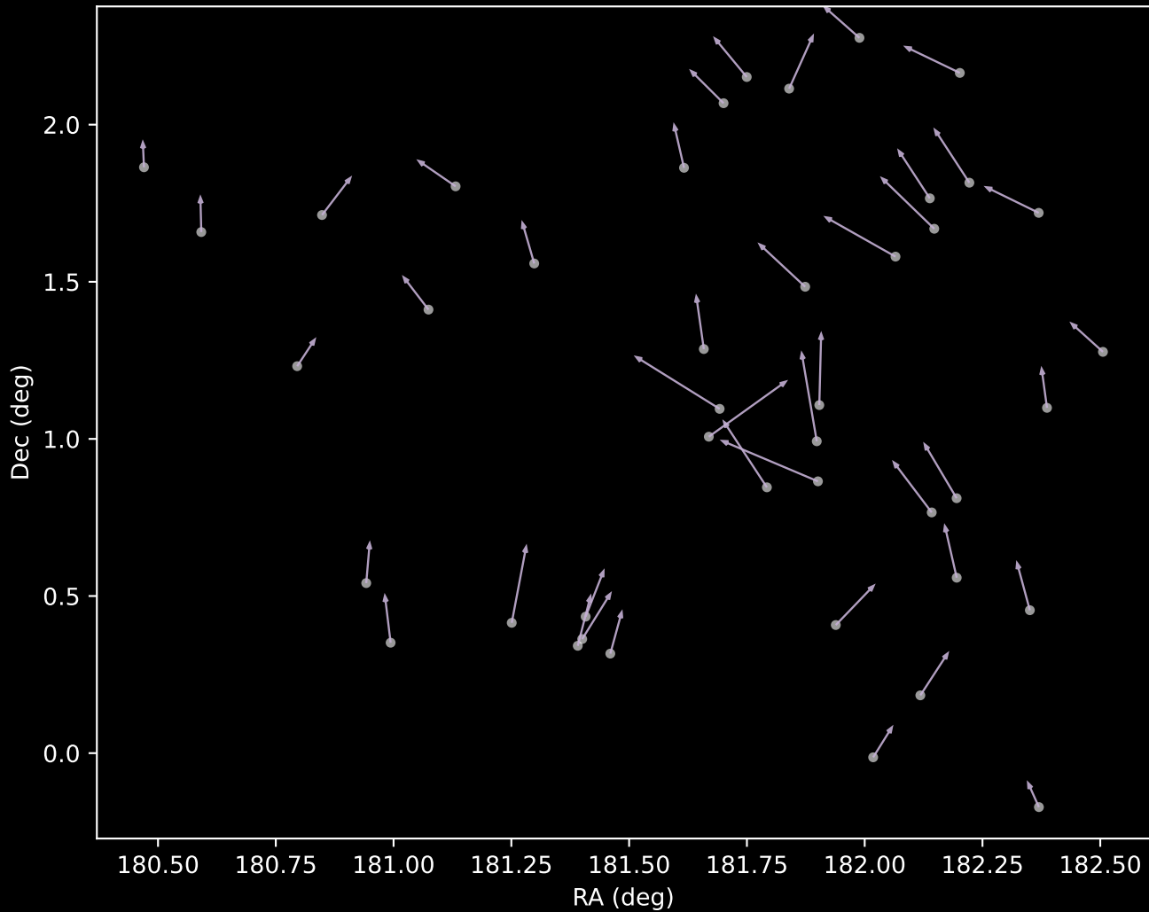
APOGEE DR17 Cluster 9 Proper Motion Vectors (n=43)
